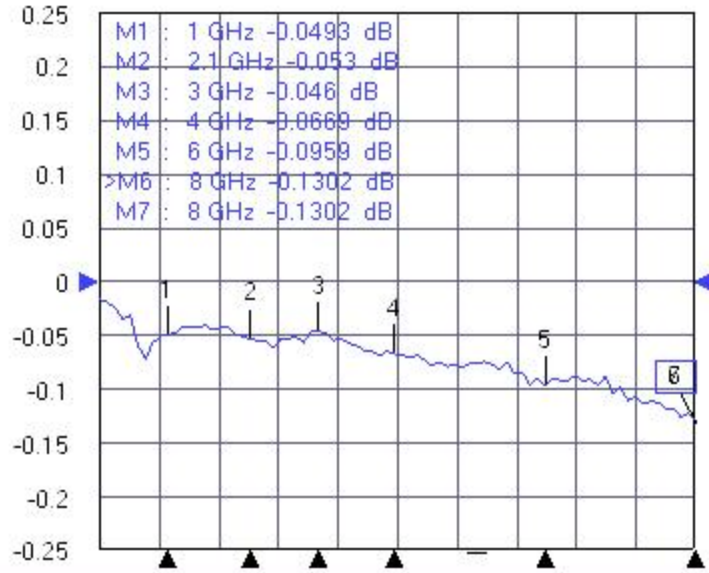
Tr3 S21 Trans LogM RefLvl: 0 dB Res: 0.05 dB/Div
