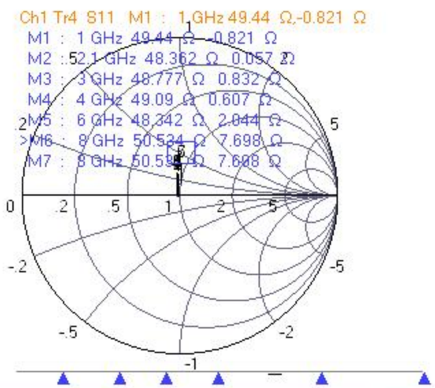
Tr4 S11 Refl Smith Imped. Scaling: 0 dB
