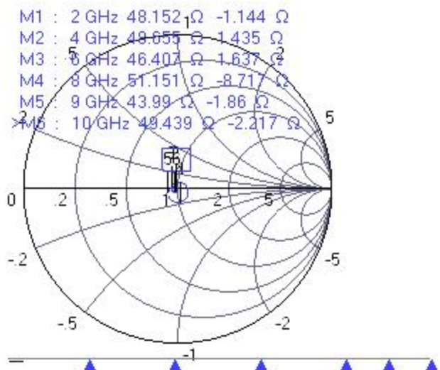
Tr4 S11 Refl Smith Imped. Scaling: 0 dB
