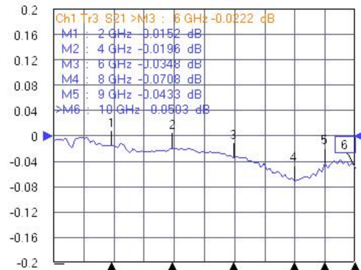
Tr3 S21 Trans LogM RefLvl: 0 dB Res: 0.04 dB/Div
