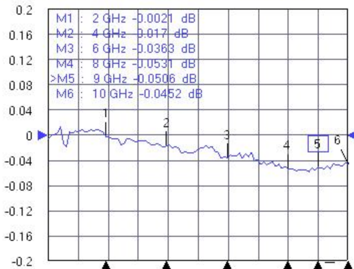
Tr3 S21 Trans LogM RefLvl: 0 dB Res: 0.04 dB/Div
