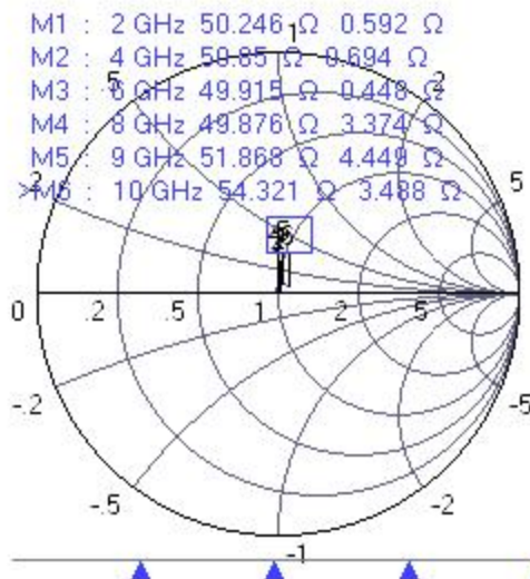
Tr4 S11 Refl Smith Imped. Scaling: 0 dB
