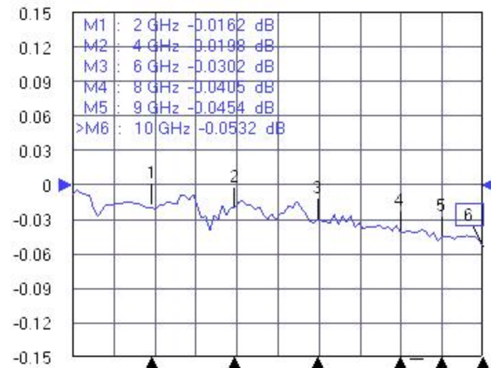
Tr3 S21 Trans LogM RefLvl: 0 dB Res: 0.03 dB/Div
