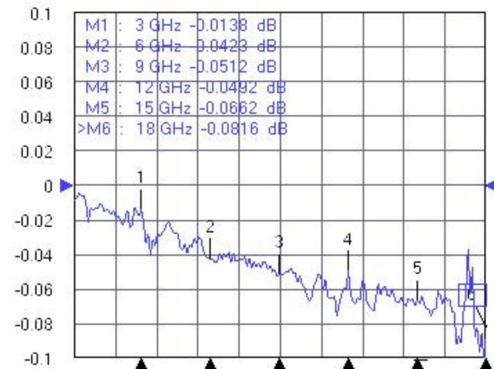
Tr3 S21 Trans LogM RefLvl: 0 dB Res: 0.02 dB/Div
