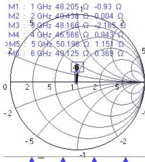
Tr4 S11 Refl Smith Imped. Scaling: 0 dB
